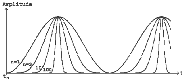
Figure 3-4 [1 - \text{Cos}(x)]^n For n = 1, 3, 10, 100
